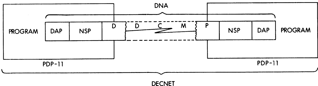
Figure 3-4 DNA Layers
